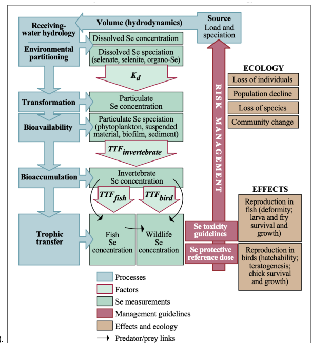
Figure 3. Conceptual illustration of the Selenium Ecosystem Scale Model (Presser and Luoma, 2010).
