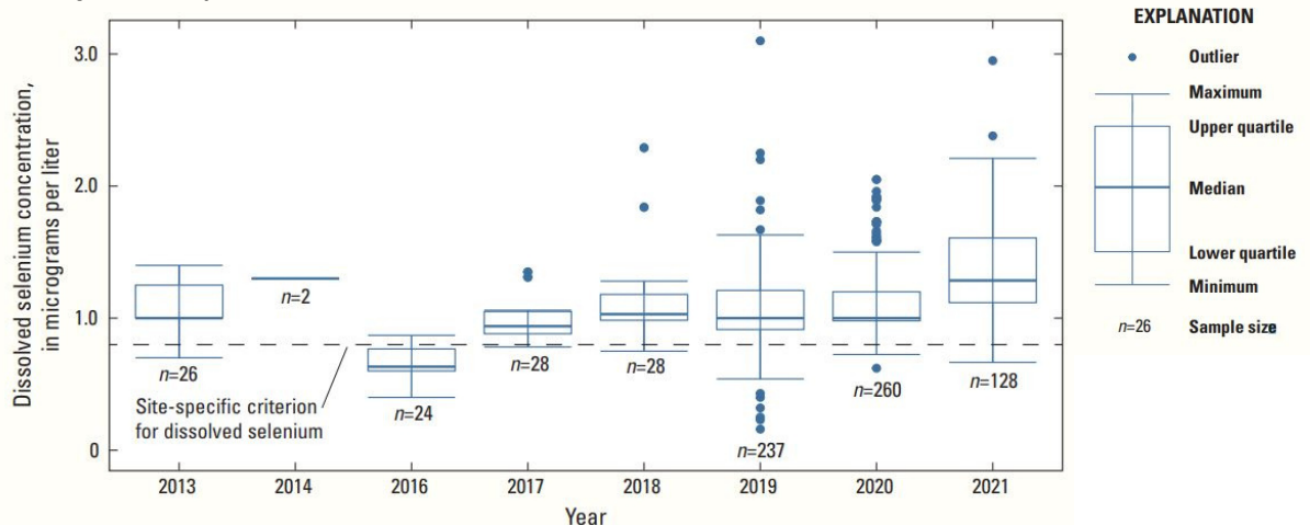
Figure 7. Dissolved selenium concentrations measured in Lake Kooconusa by the USGS, USACE, MTDEQ, and Teck Coal at sites around the International border from 2013-2021. Figure is from USGS (2022).
