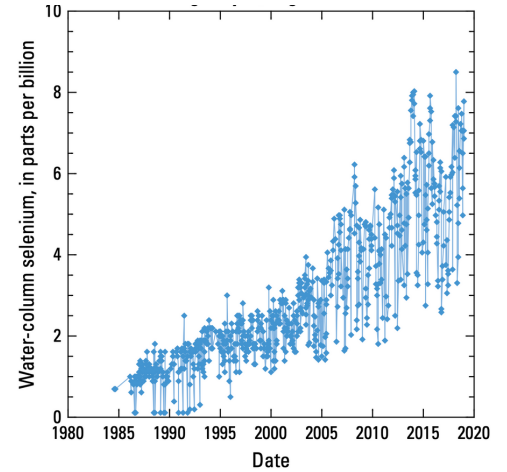
Figure 5. Water column concentrations for the Elk River at Highway 93, August 1984 to January 2019 (USGS, 2020).
